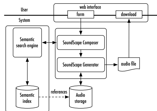
Figure 6. Overall organisation of the application.
