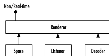
Figure 4. Soundscape Generator (SSG) structure.
