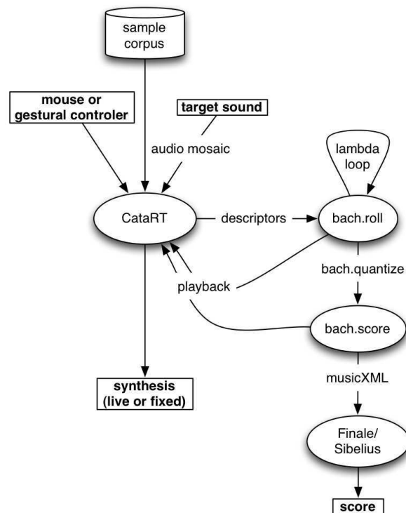
Figure 3: Flowchart for transcription, sequencing, and notation with CATART and BACH.
